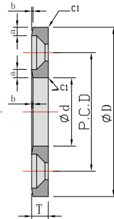
SPW WASHER STANDARD
